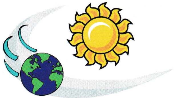
The earth revolves around the sun
