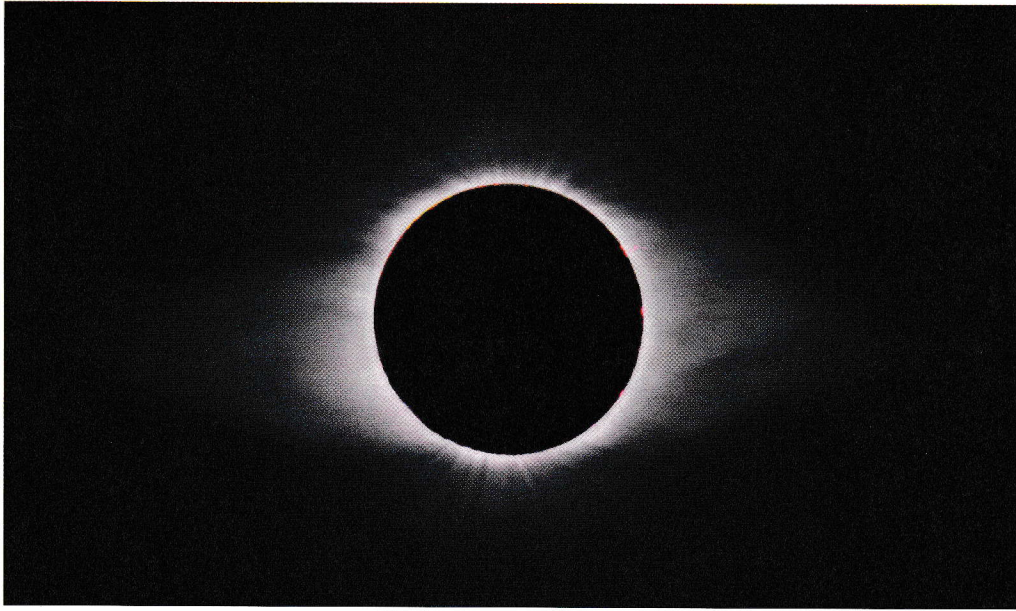
This is a picture of a solar eclipse. The dark circle in the middle is the moon, and you can see that it is blocking out most of the light that is coming from the sun.
