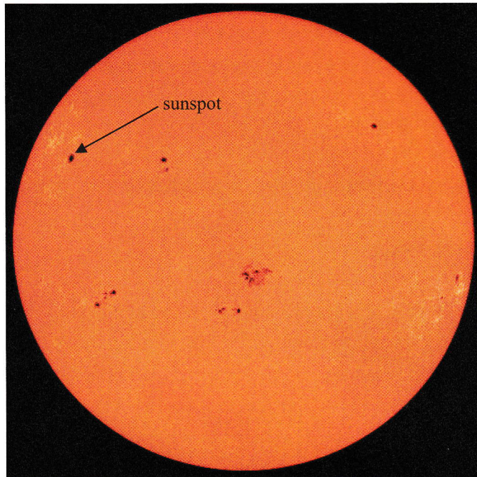
This is a picture of the sun. The dark spots are sunspots.
