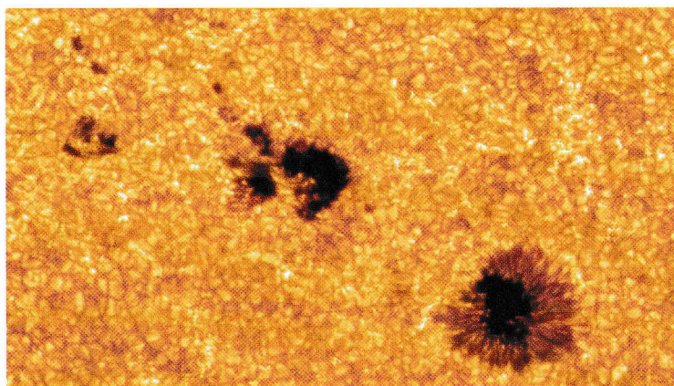
This is a close-up view of a few sunspots.
