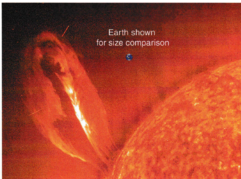
This is a photograph of a solar flare coming off the sun. The earth has been drawn in the picture to give you an idea of how big the flare is.
